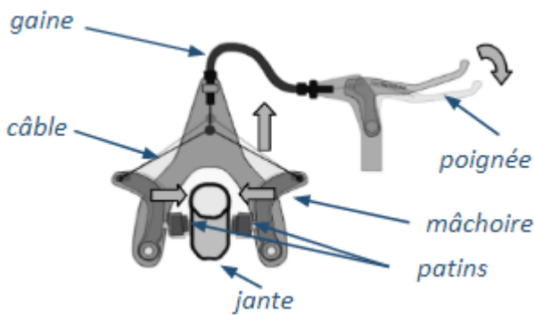
Frein cantilever
